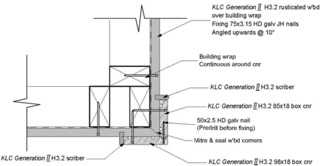
D1.10 Direct Fix, External Box Corner
