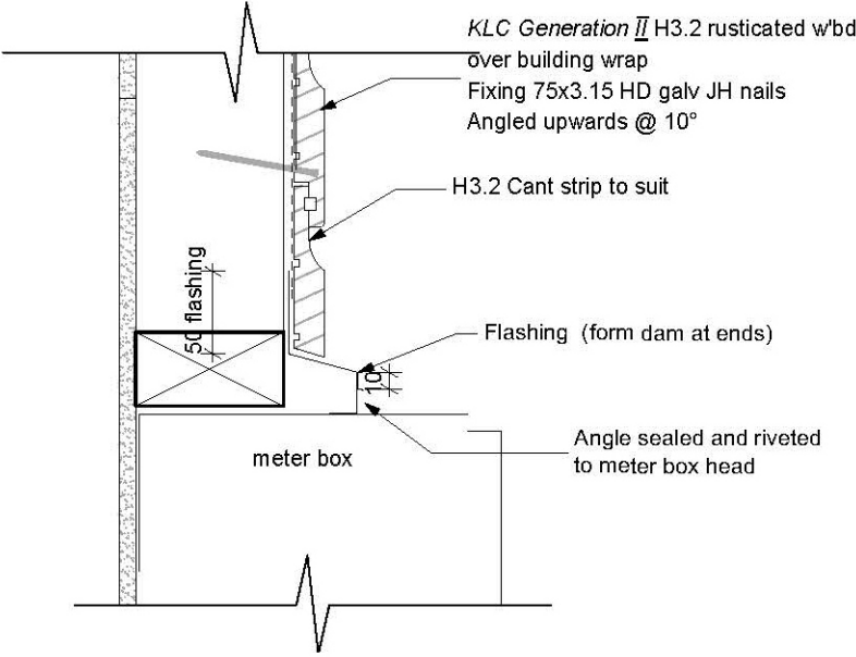
D1.13 Direct Fix, Meter Box Head
