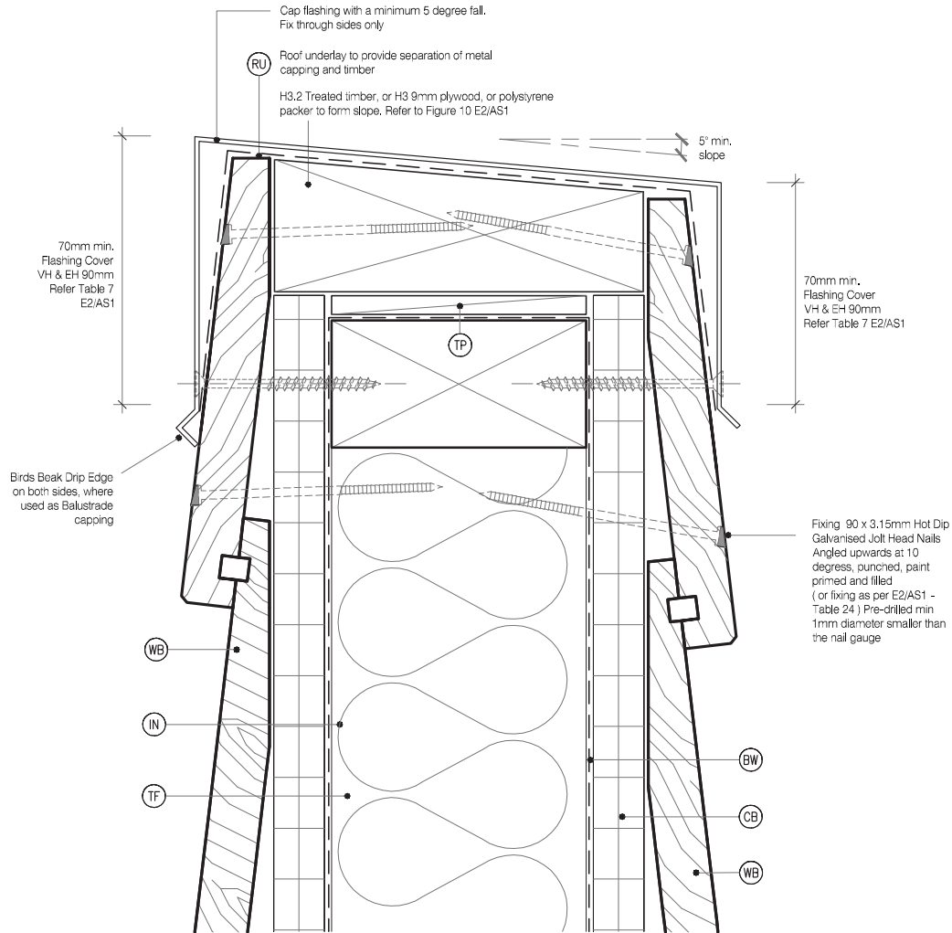
E2/AS1 Section 6.0 PARAPETS Parapets require a drained cavity for claddings
