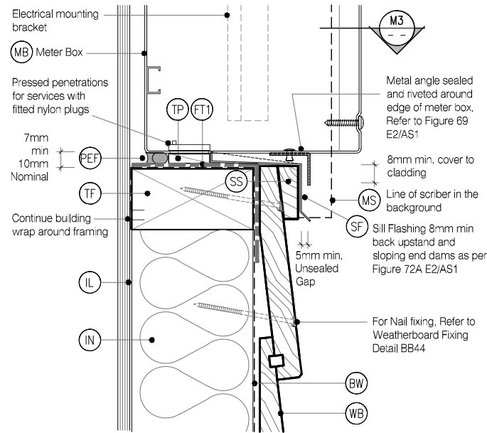
M2 METER BOX SILL BB31 Direct Fix - Bevel Back Weather Boards SCALE 1:2 @ A1, 1:4 @ A3
