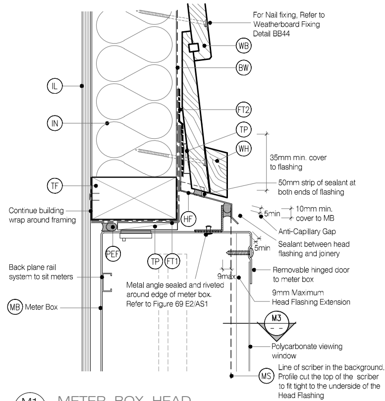
M1 METER BOX HEAD BB30 Direct Fix - Bevel Back Weather Boards SCALE 1:2 @ A1, 1:4 @ A3
